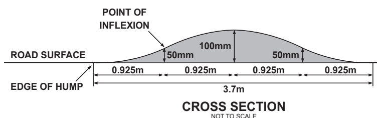
Fig 4.7 Cross-section and plan view of a sinusoidal hump
