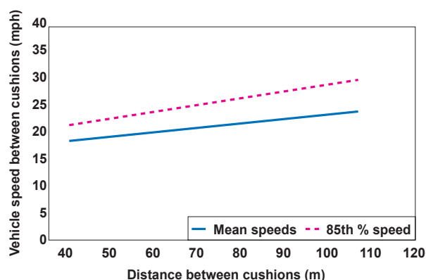
Fig. 4.17 Vehicle speeds between cushions
