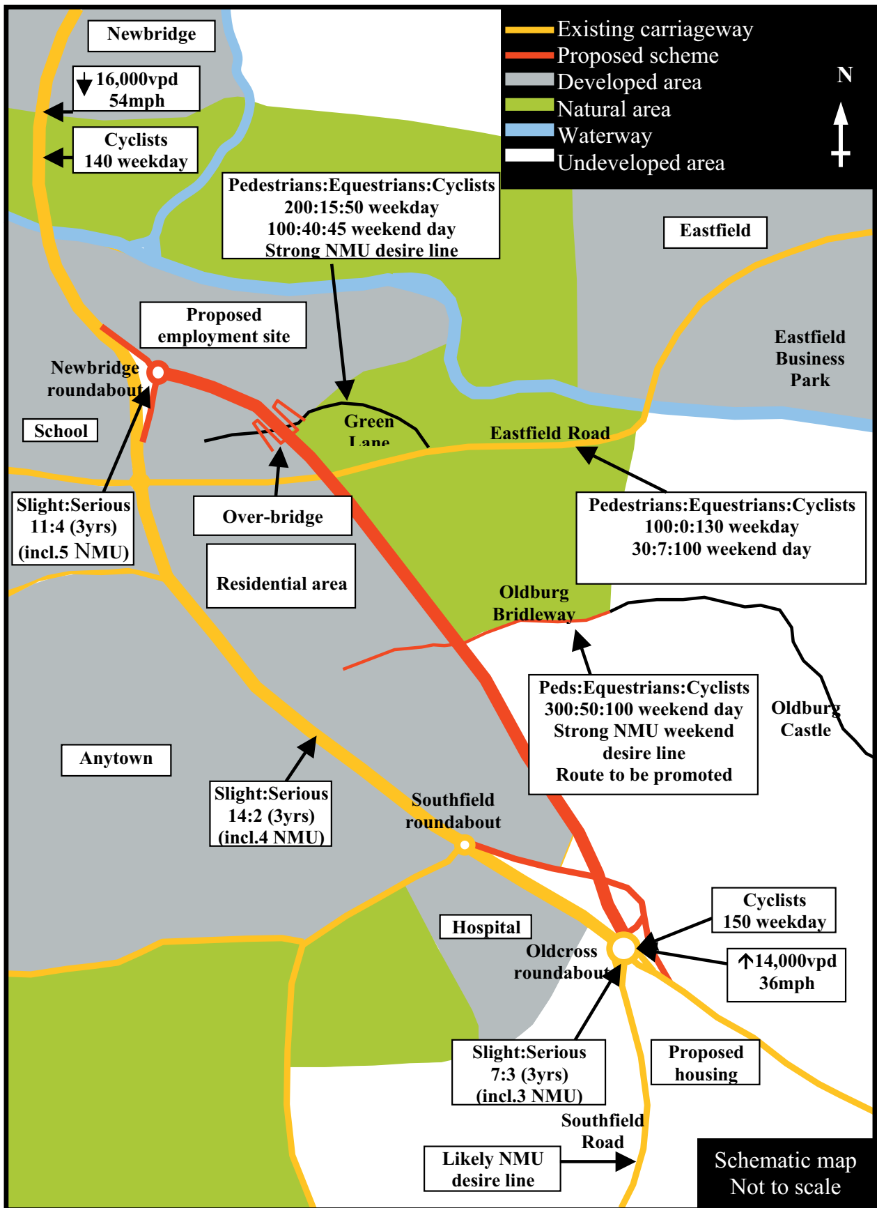
Figure 1: Schematic Map showing proposed scheme and contextual information
