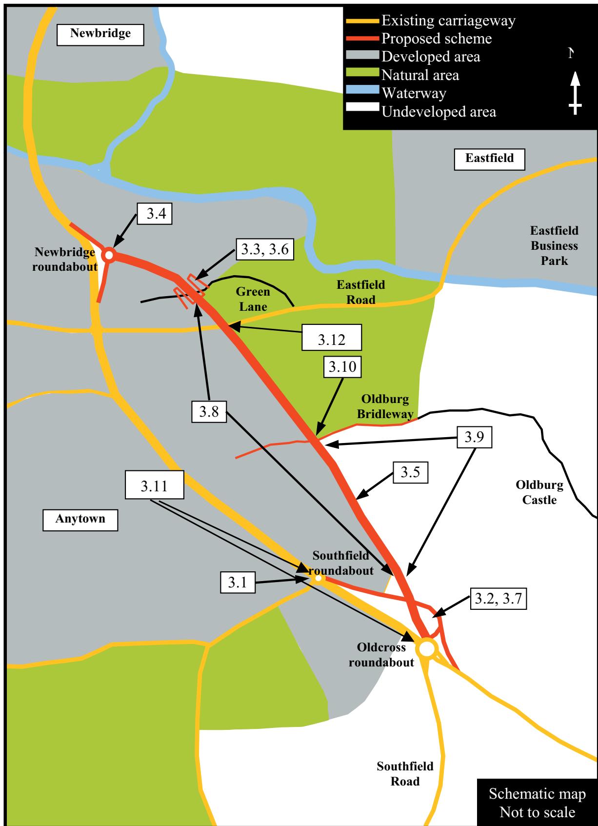
Figure A – Layout Plan with references to Issues/Actions Taken (NB numerical references refer to numbering in Section 3 of report)
